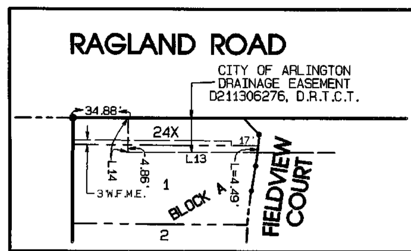
DRAINAGE EASEMENT DETAIL
